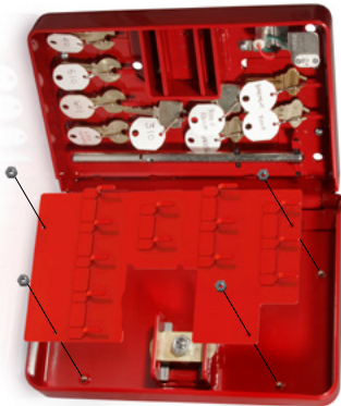
Expansion Panel Mounting Illustration
