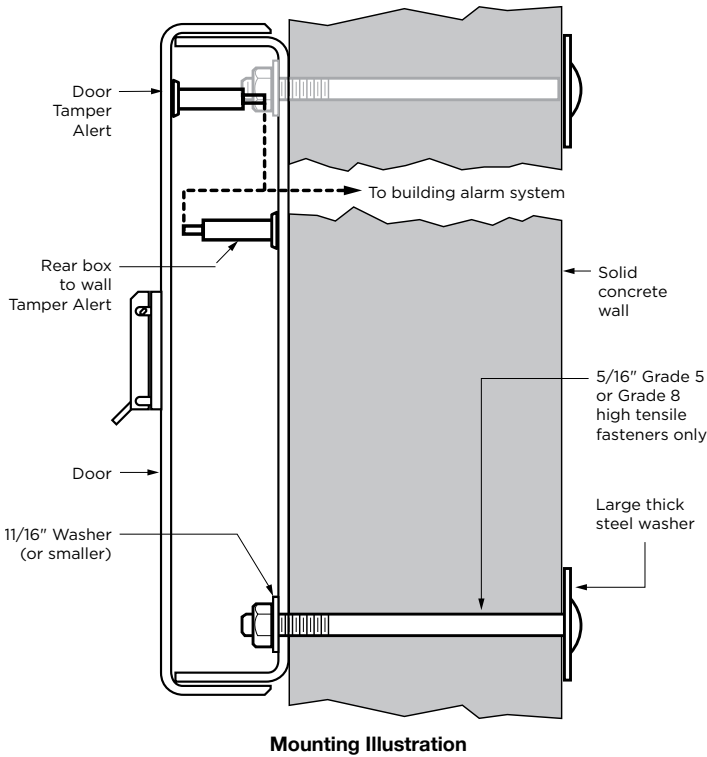
Mounting Illustration
